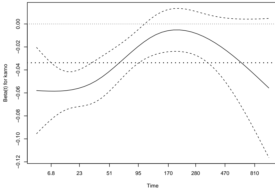
Figure 1: Solid line = the estimated effect if Karnofsky score, versus time, in the Veteran's cancer data set, as estimated by cox.zph , along with confidence intervals. Dotted lines are the overall estimate from a Cox model with karno as a time-fixed effect, and a reference line at 0.
